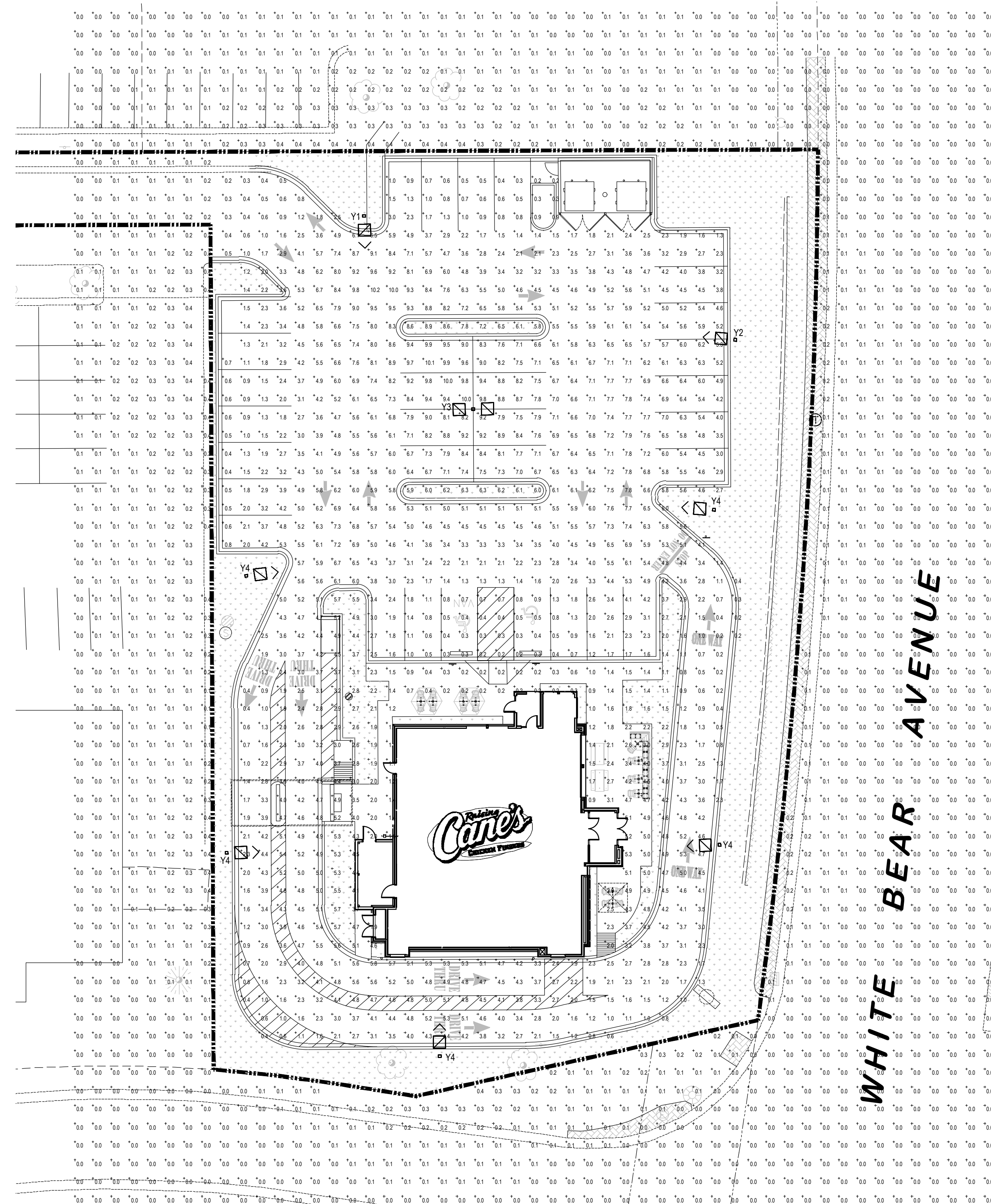
PHOTOMETRIC SITE PLAN SCALE 1" = 20'-0"
